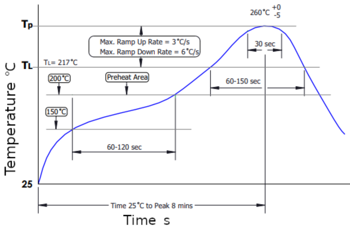
Figure 4: Recommended soldering profile for OEM TT-SF1
