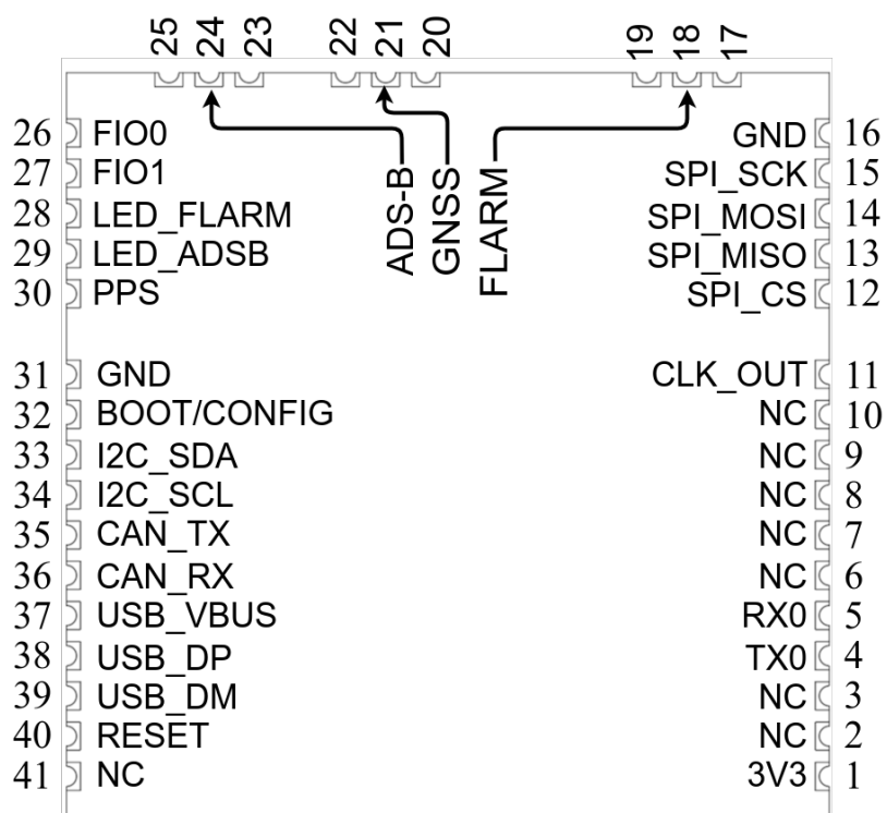
Figure 1: Pin arrangement of OEM TT-SF1.
