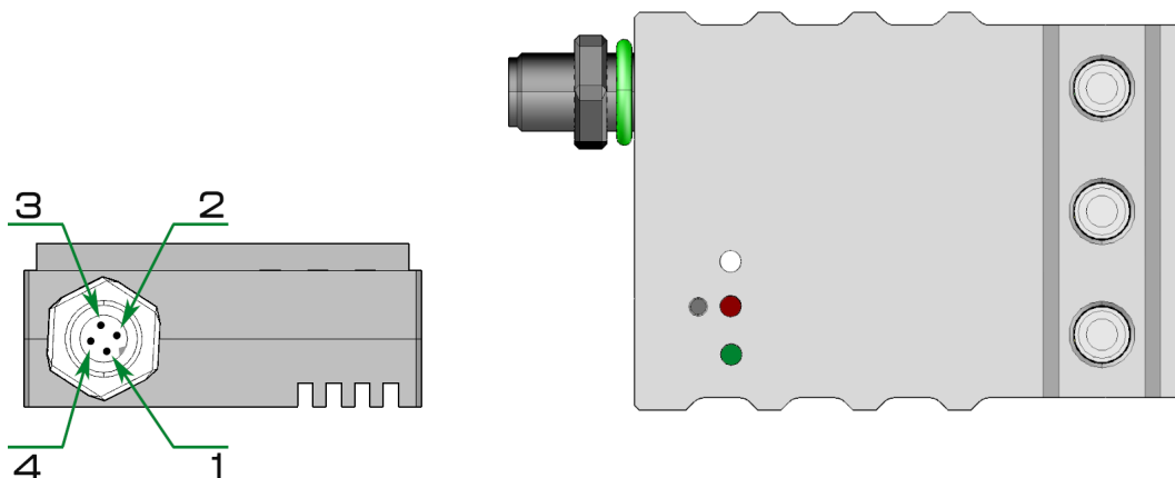
Figure 1: Appendant drawing of Transceiver TR-1F .
