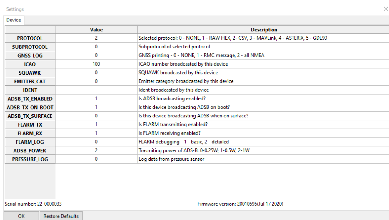
Figure 8: Settings window
